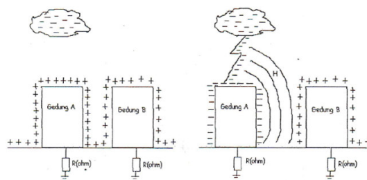
Gambar 6. Mekanisme Coupling Inductive
