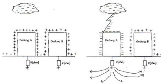
Gambar 5. Mekanisme Coupling Resistive
