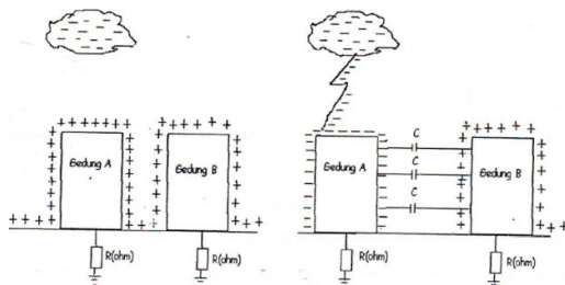
Gambar 7. Mekanisme Coupling Capacitive
