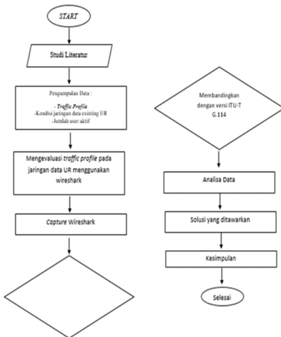
Gambar 1. Flowchart Penelitian
