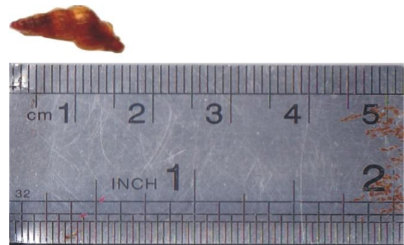
Gambar 3. Oncomelania hupensis
