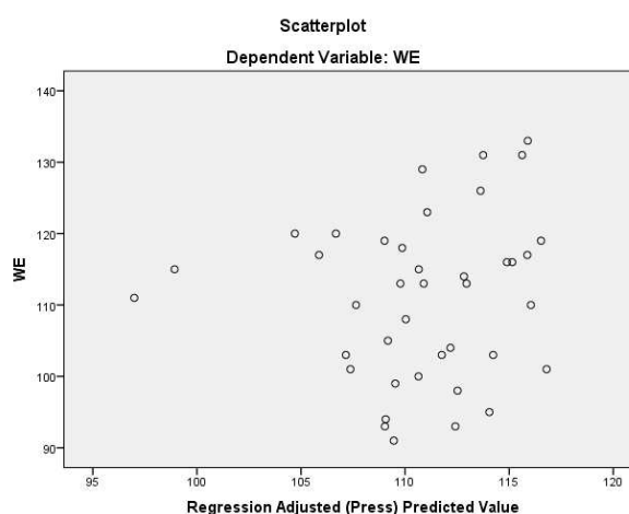
Gambar 1. Scatter Plot Sebaran Data Prediktor terhadap Work Engagement
