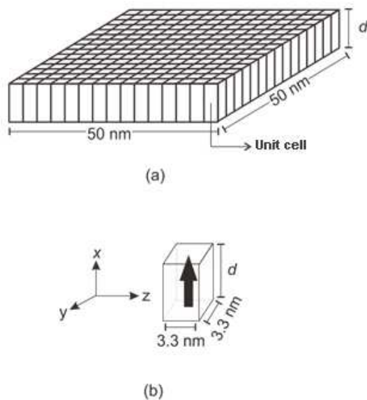
Figure 1. (a) Nano-dot Barium-ferrite, (b) unit cell.
