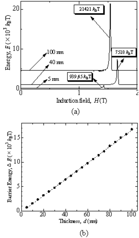
Figure 3. (a). The energy of Barium-ferrite nano-dot for three different thicknesses 5 nm, 40 nm, and 100 nm, (b). The barrier energy of Barium-ferrite nano-dot for various thicknesses at room temperature.
