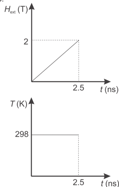
Figure 2. Reduce Barrier Writing scheme.
