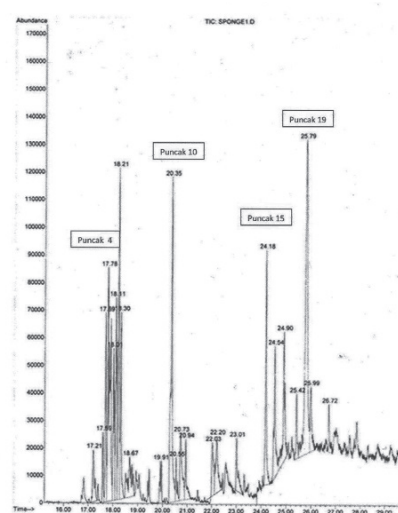
Gambar 2: Kromatogram gas F_B
