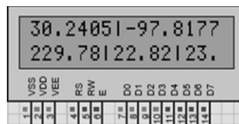
Fig 7. Depth and temperature value displayed in LCD
