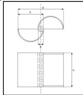
Gambar 3. Turbin Angin Savonius
