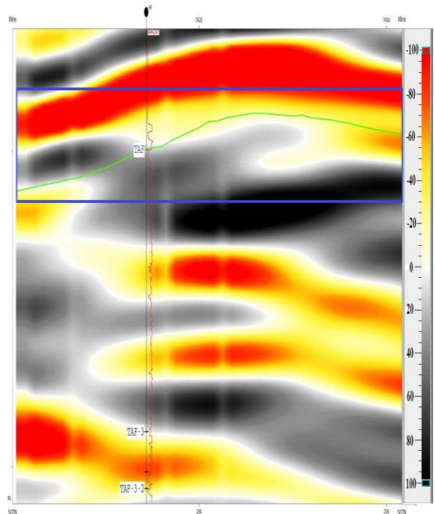
Gambar 5 Penampang seismik near angle stack .
