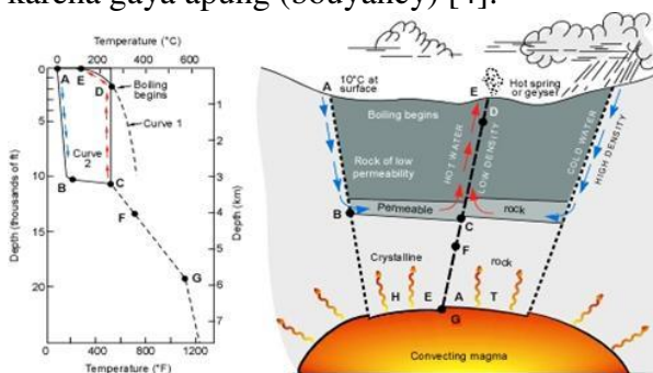
Gambar 1. Model Sistem Geotermal [4]
