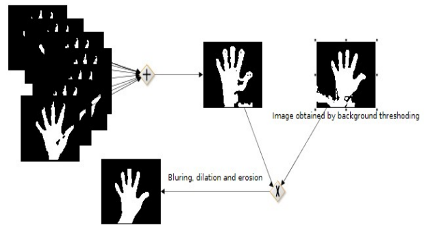
Gambar 5. Segmentasi Filter[3]
