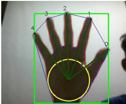
Figure 5. Gesture Extraction
