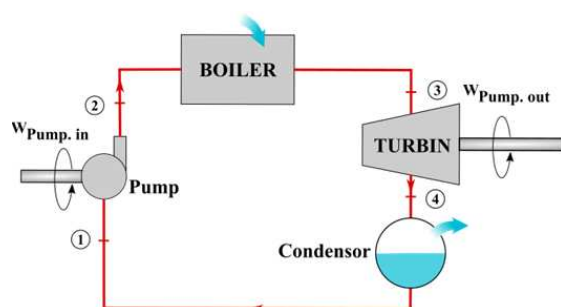
Gambar 2 Siklus Rankine Ideal
