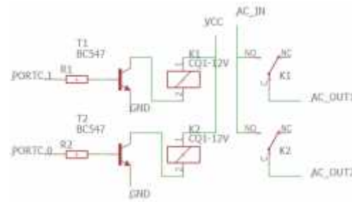
Gambar 3.5 Skema Rangkaian Driver Relay
