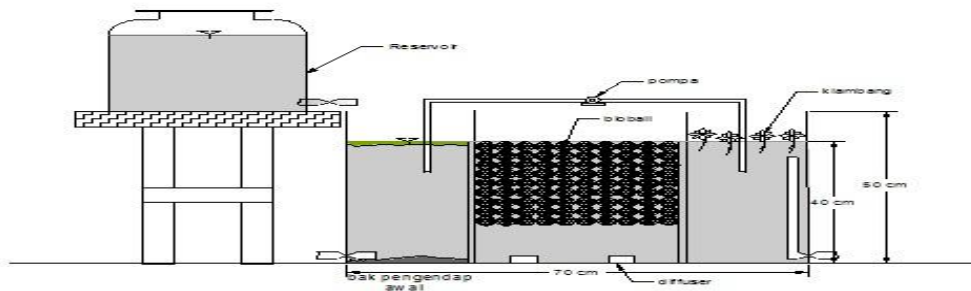
Gambar 1. Rancangan reaktor penelitian biofilter aerob
