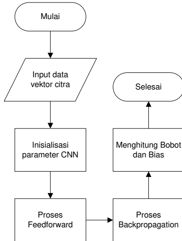
Gambar.8. Alur Proses Training
