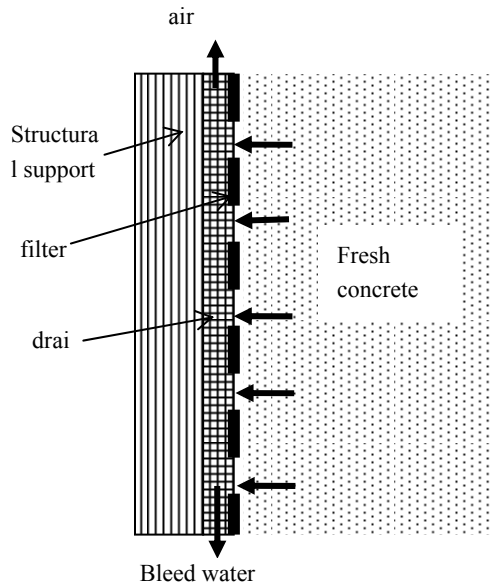
Figure 1. General elements of a CPF system (Price, 2000)
