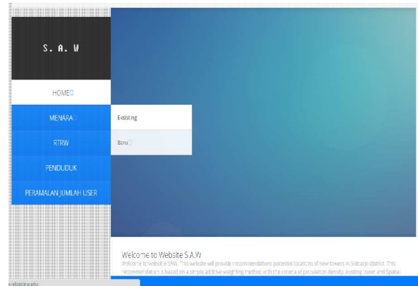
Gambar 4. Menu Website
