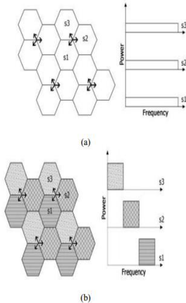
Gambar 1. Conventional Frequency Reuse (a) Frequency Reuse factor 1 (b) Frequency reuse Factor 3
