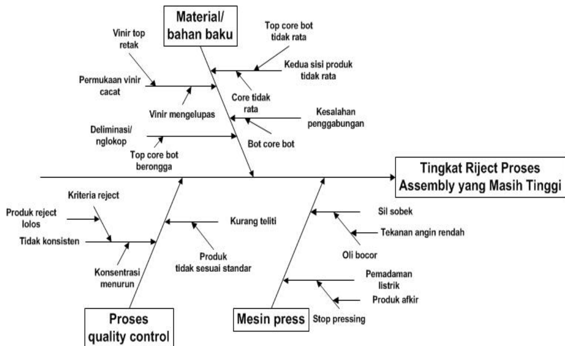
Gambar 2 Diagram Fishbone
