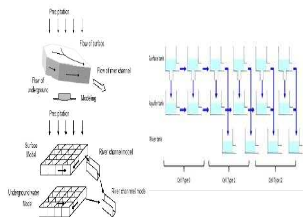
Gambar 1 Skema Model IFAS
