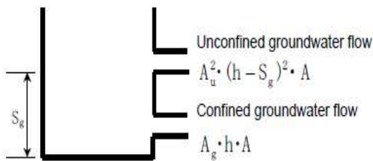
Gambar 3 Konsep Underground Water Model Sumber : Fukami, 2009
