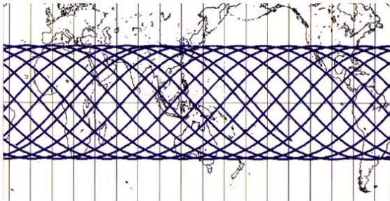
Gambar 1. Orbit satelit TRMM (Sumber: BBTMC, 2010)
