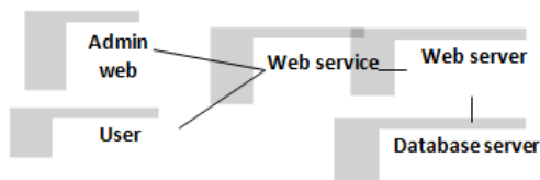
Gambar 4 Deployment Diagram
