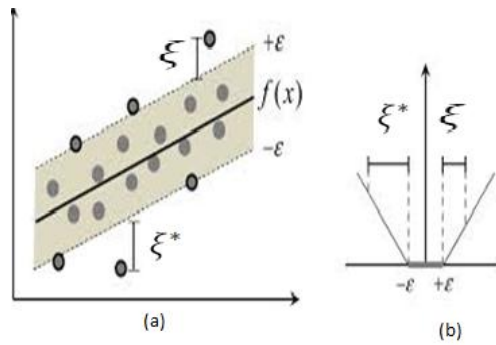
Gambar 2. (a) SVR output, dan (b) \epsilon -insensitive loss function
