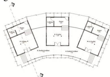
Gambar 26 Denah Retail Komersil Fasilitas Jajanan
