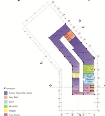
Gambar 25 Denah Lantai Tiga
