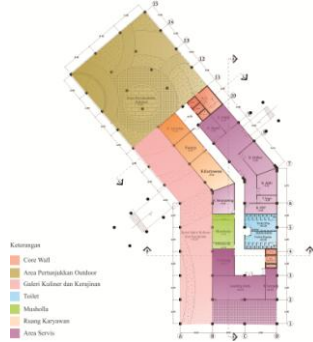
Gambar 22 Denah Lantai Dasar
