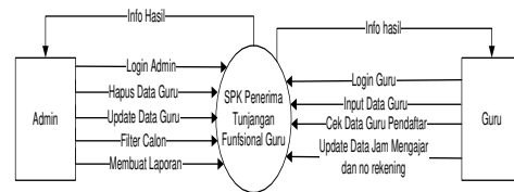
Gambar 1 Context Diagram
