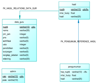
Gambar 4 Physical Data Model (PDM)
