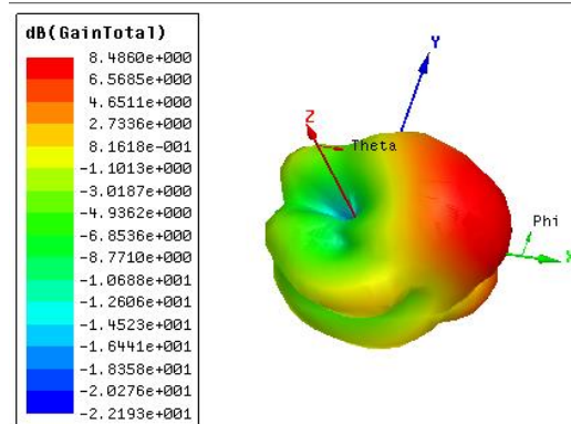
Gambar 3.7 3D Polar Plot Gain Hasil Optimasi Antena Mikrostrip H-Shaped 4 Elemen Substrat Duroid ( \varphi = 0^0 - 360^0 ; \theta = 0^0 - 360^0 )
