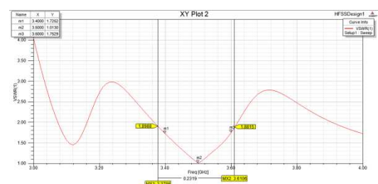
Gambar 3.2 VSWR Hasil Optimasi Antena Mikrostrip Slot H-Shaped 4 Elemen Substrat FR4_epoxy
