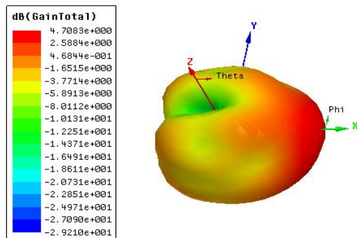
Gambar 3.5 3D Polar Plot Gain Hasil Optimasi Antena Mikrostrip H-Shaped 4 Elemen Substrat FR4_epoxy ( \varphi = 0^0 - 360^0 ; \theta = 0^0 - 360^0 )
