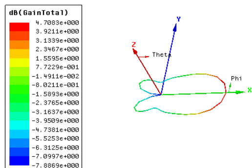
Gambar 3.6 3D Polar Plot Gain Hasil Optimasi Antena Mikrostrip H-Shaped 4 Elemen Substrat FR4_epoxy ( \varphi = 0^0 - 360^0 ; \theta = 90^0 )
