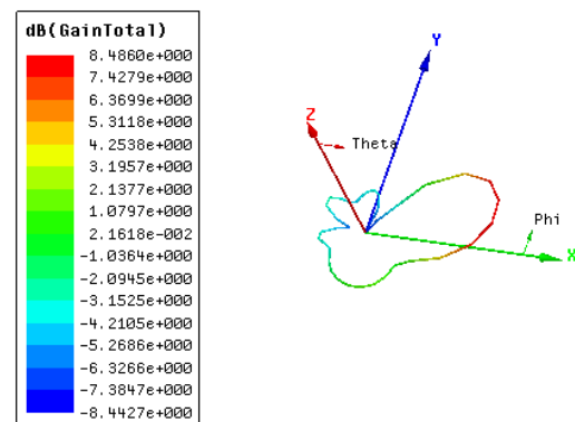
Gambar 3.8 3D Polar Plot Gain Hasil Optimasi Antena Mikrostrip H-Shaped 4 Elemen Substrat Duroid ( \varphi = 0^0 - 360^0 ; \theta = 70^0 )
