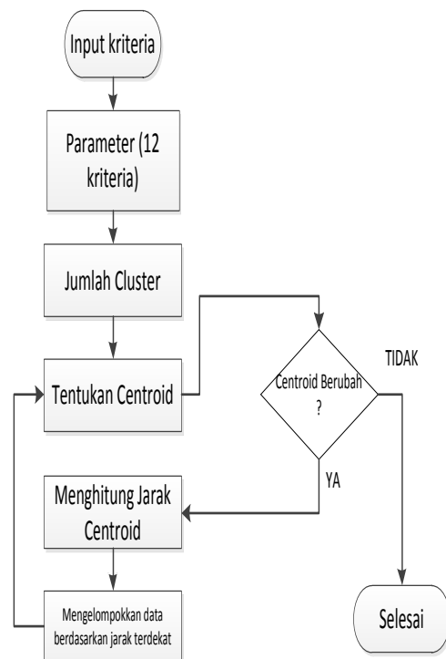
Gambar 2 Proses Algoritma K-Means Clustering
