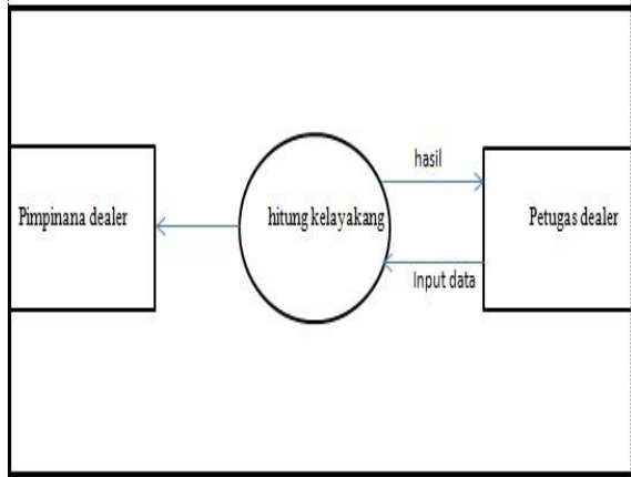
Gambar 3 Dfd Context
