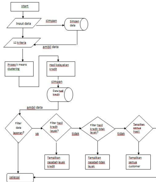
Gambar 5 Flowchart Program
