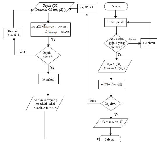
Gambar 1. Flowchart metode Dempster Shafer
