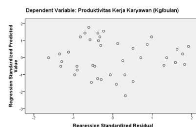
Gambar 3. Diagram Scatterplot
