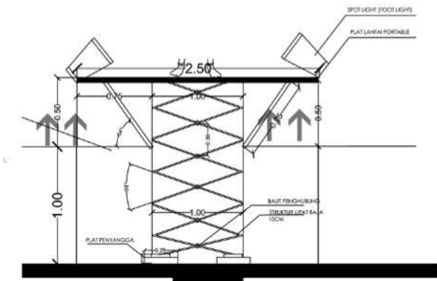
Gambar. 2.29 Detail Stage (tematik eventual)
