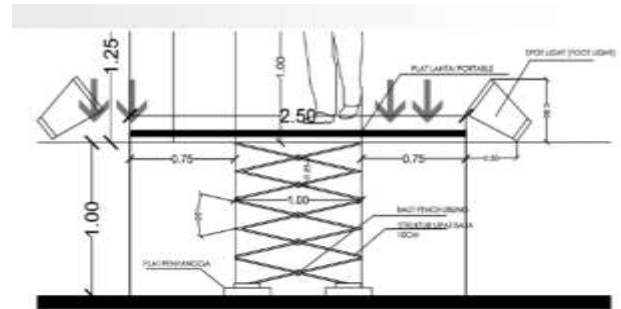
Gambar. 2.28 Detail Stage (daily activity)
