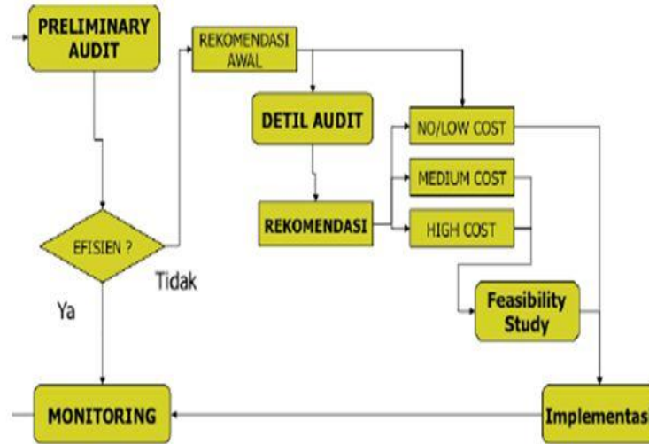
Gambar 2. Diagram alur audit energi
