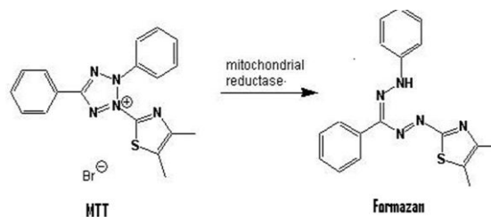
Gambar 9. Reaksi reduksi MTT (Mosmann, 1983)
