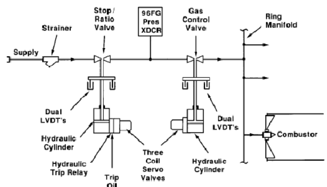
Gambar 2. Sketsa sistem kendali suplai bahan bakar gas [1]
