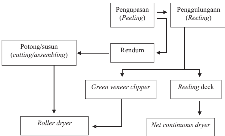
Gambar 1. Alur proses pengupasan venir Figure 1. Flow chart of veneer peeling
