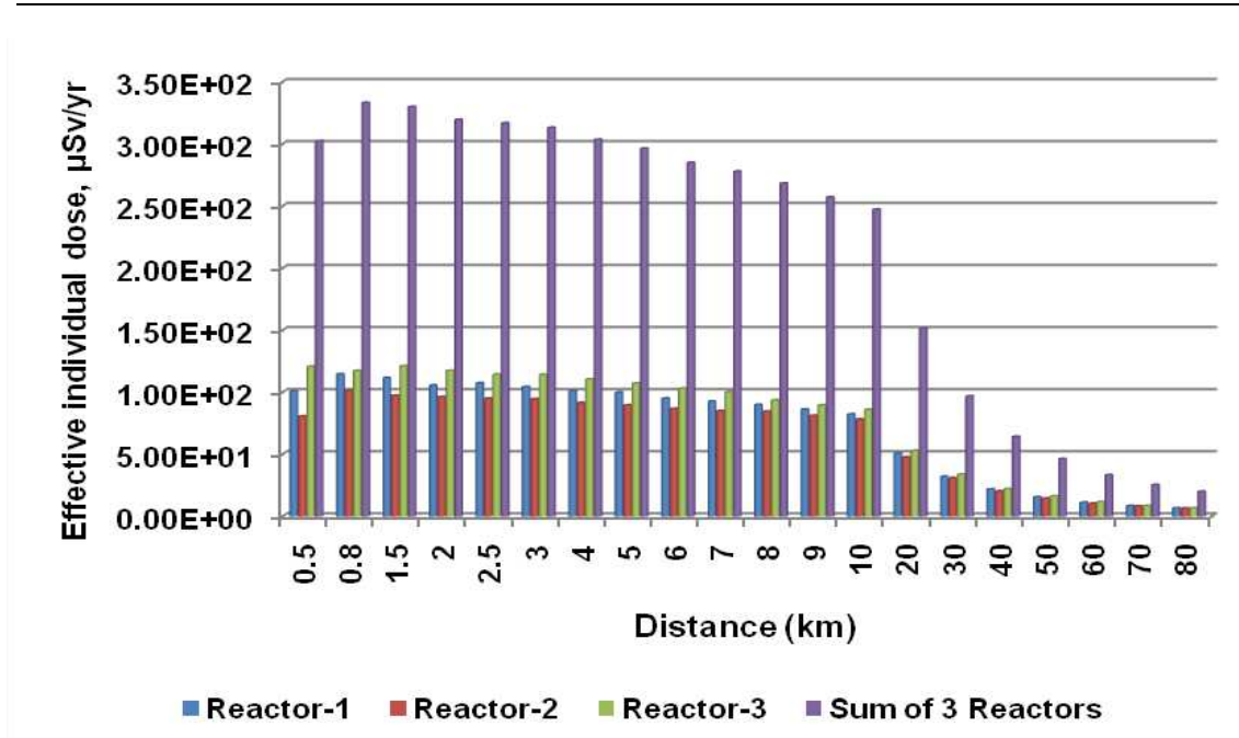
Figure 2. The individual effective doses from each of the PWRs as a function of the radius from the reactor
