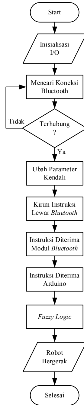
Gambar 8. Flowchart sistem
