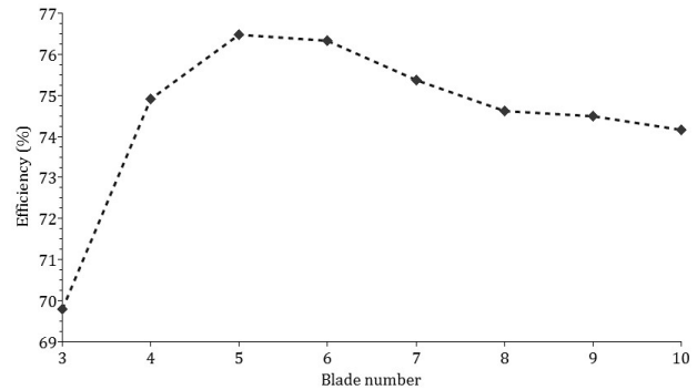
Fig. 7 Dependence of efficiency on blade number
