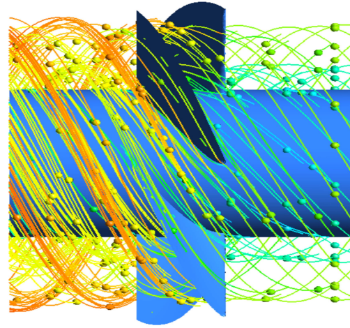
Fig. 17 Axial flow turbine stream line flow
