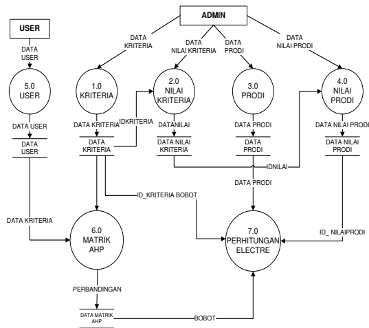
Gambar 3 Model Level 0
