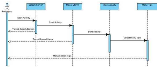
Gambar 7. Sequence Diagram Tips
