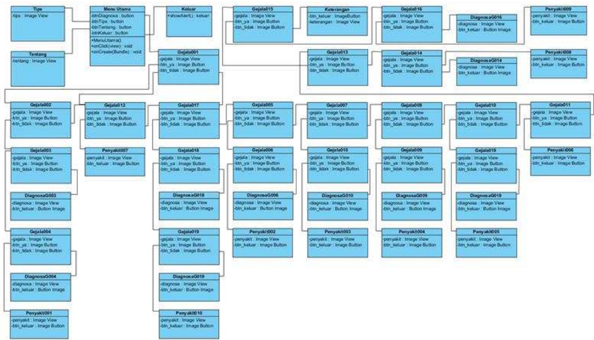
Gambar 5. Class Diagram
