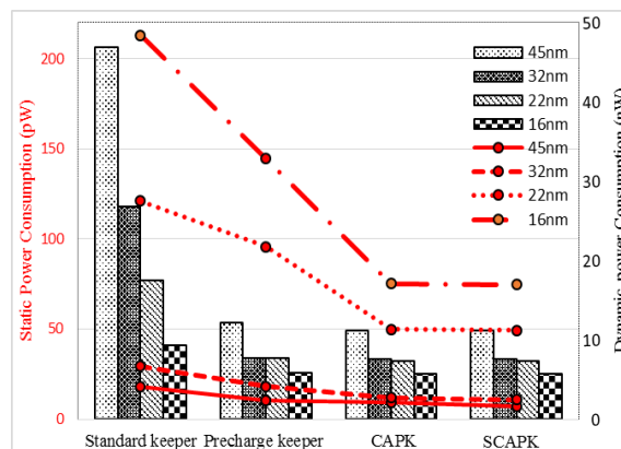
Figure 9. Two input AND gate simulation result for static and dynamic power consumption
