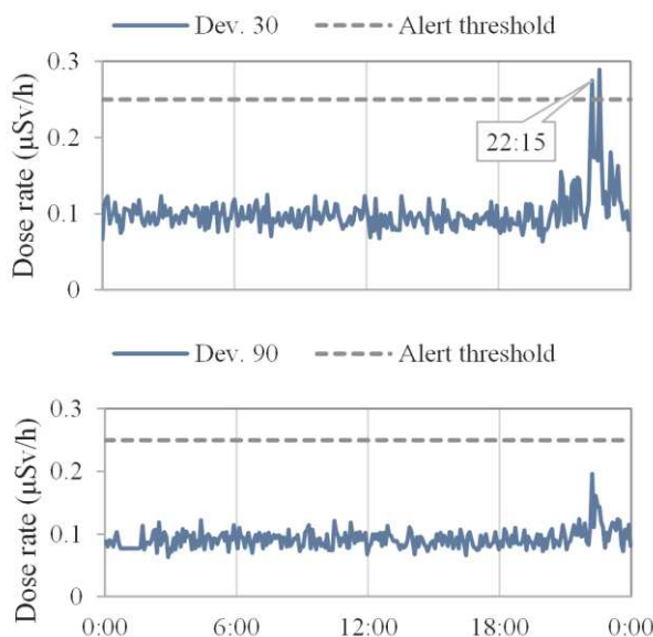
Fig. 5. Air dose rate profiles at locations 30 and 90 during operation of medical isotope production facility
