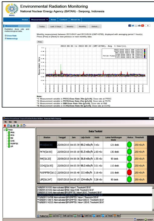
Fig. 1. Web interface and software at the control center of the environmental radiation monitoring system.
