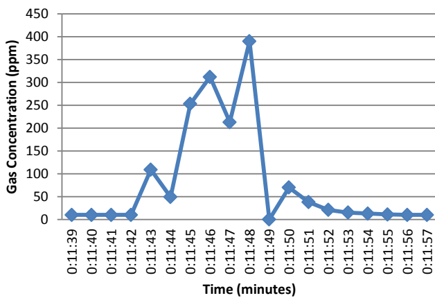
Fig. 7. Graph of gas leakage detection.
