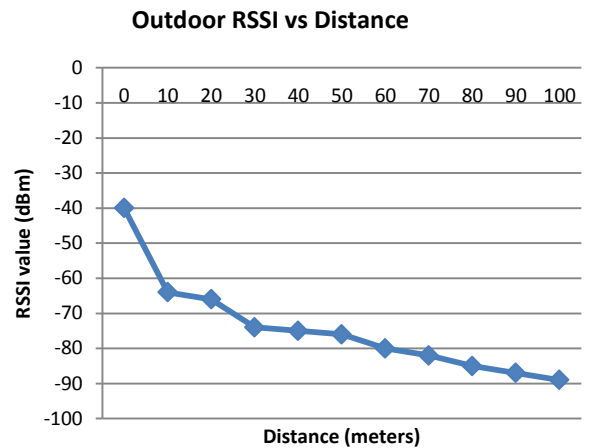
Fig. 6. Graph on receive signal strength indicator of Zigbee module versus distance outdoor of the building.
