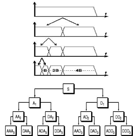
Fig. 2 : Structure of the discrete wavelet filter bank [17]
