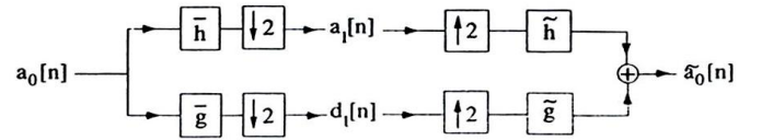
Fig. 1 : Mechanism of the input signal is filtered at decomposition and re-incorporated in the reconstruction [16]
