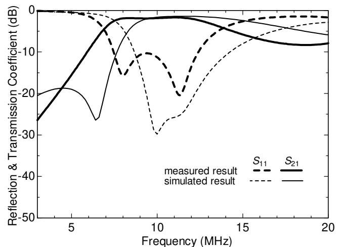
Fig. 6. Comparison of measured and simulated results for 0.4mm gap separation
