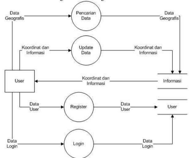
Figure 4. DFD Digram
