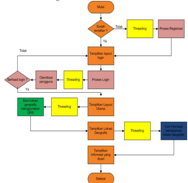
Figure 5. Flowchart
