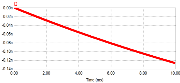
Fig. 5. Simulation results of insulation resistance equivalent circuit under normal conditions
