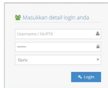
Gambar 4. Form Login
