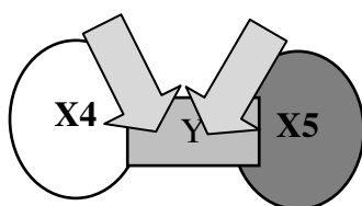
Gambar 1: Desain Penelitian
