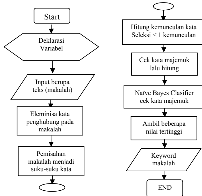
Gambar 3. Flowchart Program
