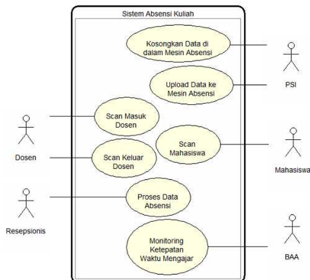
Gambar 3. Use Case Sistem Absensi Kuliah
